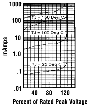
Typical Reverse Characteristics
